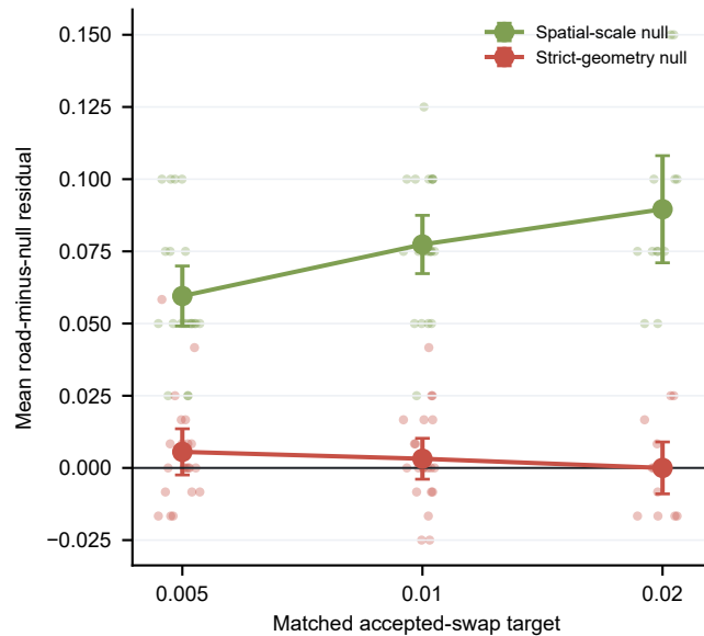
b Matched-intensity defense on R67 subset
