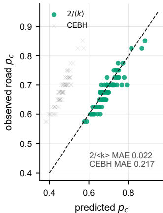
a Zero-fit p_c = 2/\langle k \rangle
