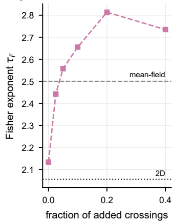
d Exponent rises with crossings
