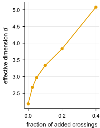
c Dimension rises with crossings
