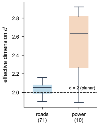
b Roads 2D, power not
