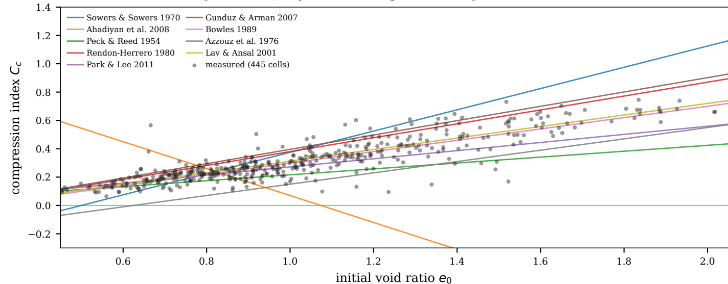
Nine published e_0 -only correlations against an independent 445-cell dataset
