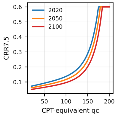
(c) Liquefaction resistance
