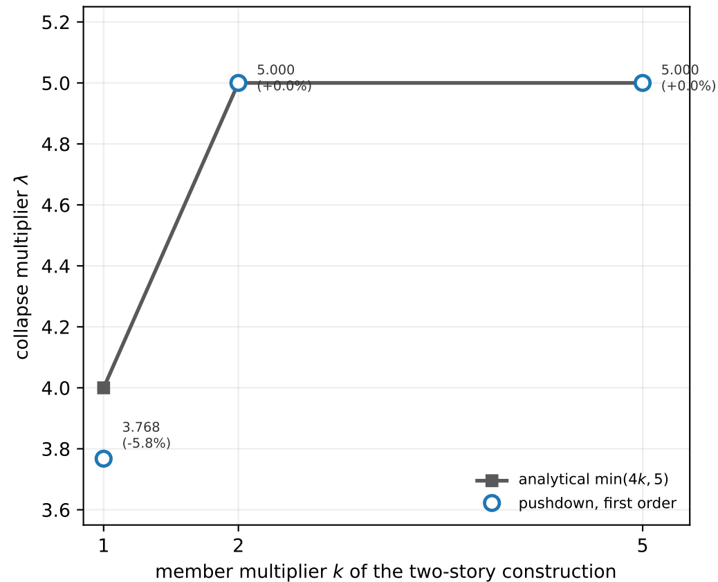
(c) Solver verification against the analytical boundary
