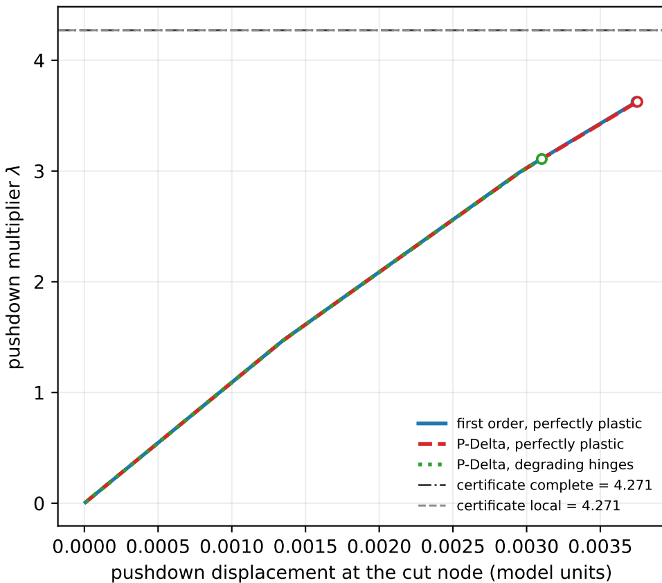
(a) Exact case: certificate margin +0.935
