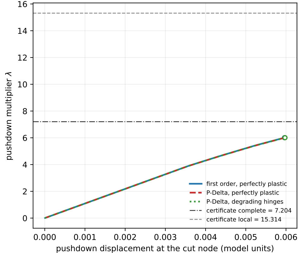
(b) Inexact case: certificate margin -8.537
