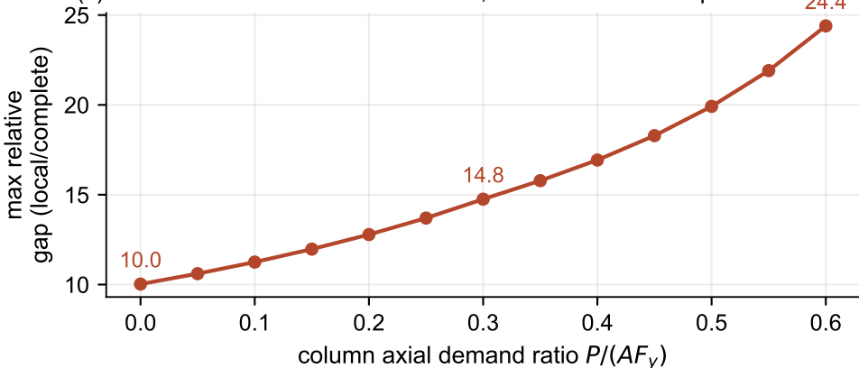
(c) Interaction does not create failures; it scales the consequence of a failure
