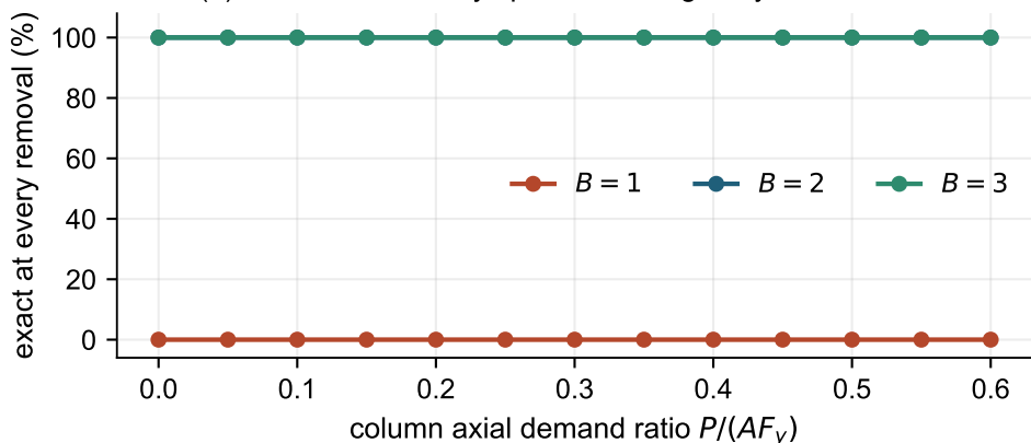
(a) The screen-validity split is unchanged by axial demand
