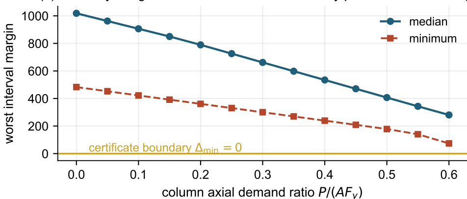
(b) Multi-bay margins fall with axial demand but stay positive in all 45 designs
