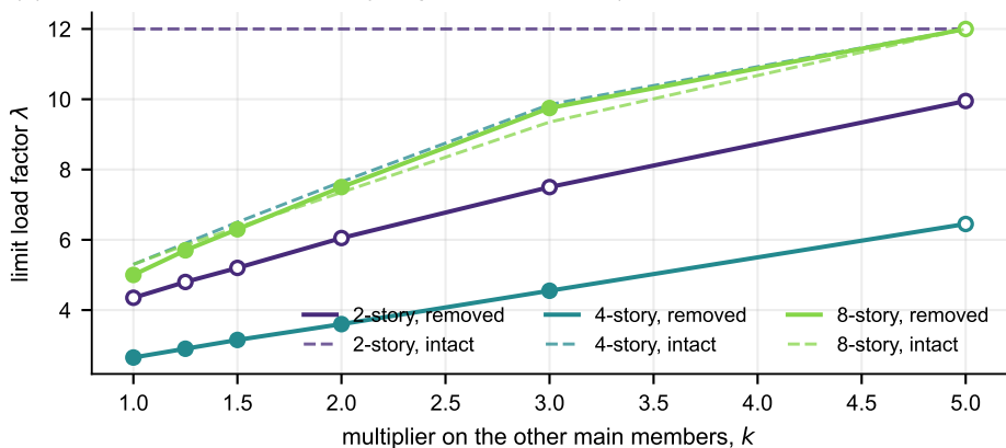
(a) Source-traceable SAC/Elkady--Lignos control runs (open marker: censored at the load ceiling)
