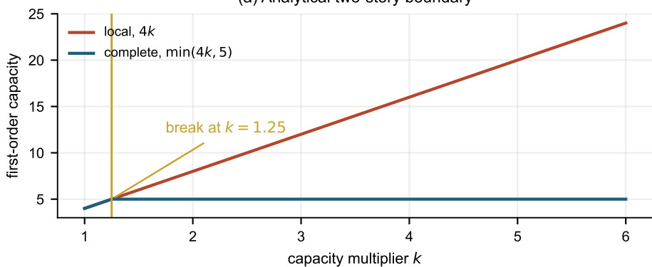
(a) Analytical two-story boundary
