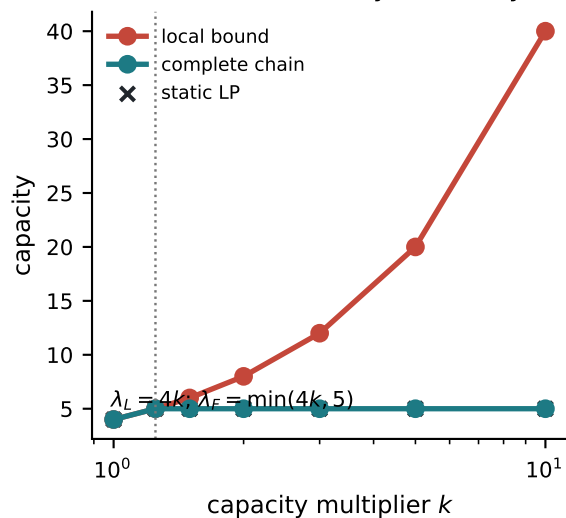
(c) Exact product-one redistribution
