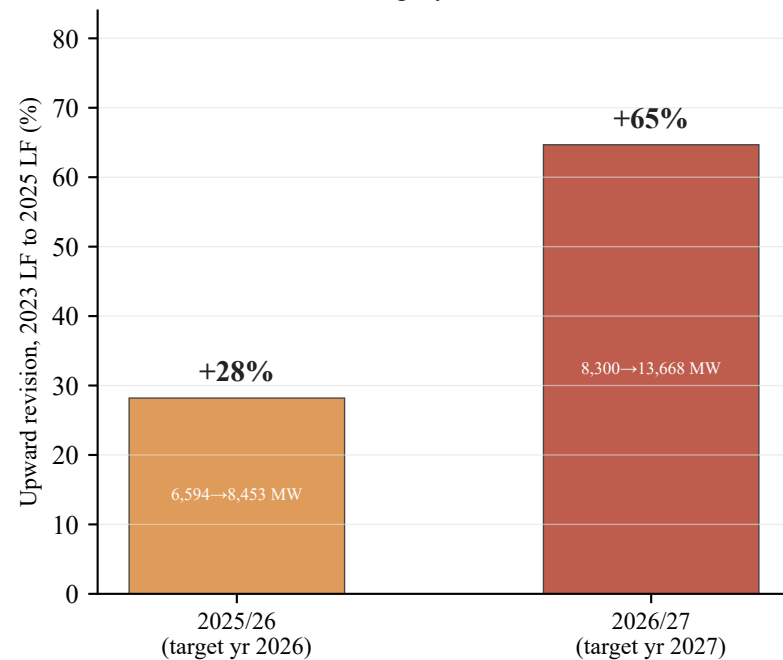
(b) Vintage escalation for the two BRA-committed target years
