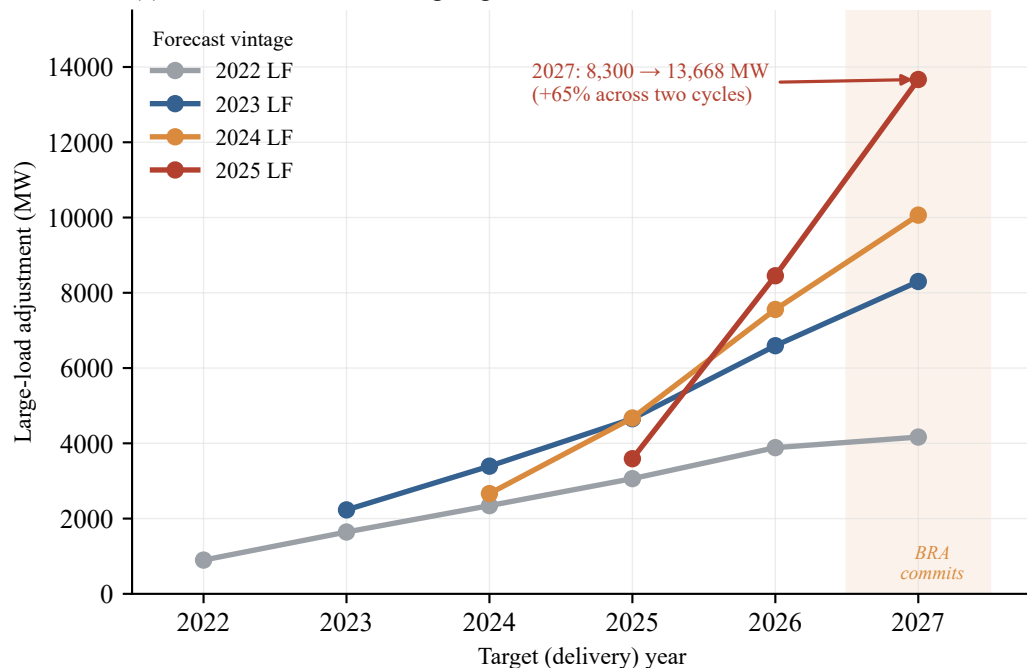
(a) The forecast is a moving target
