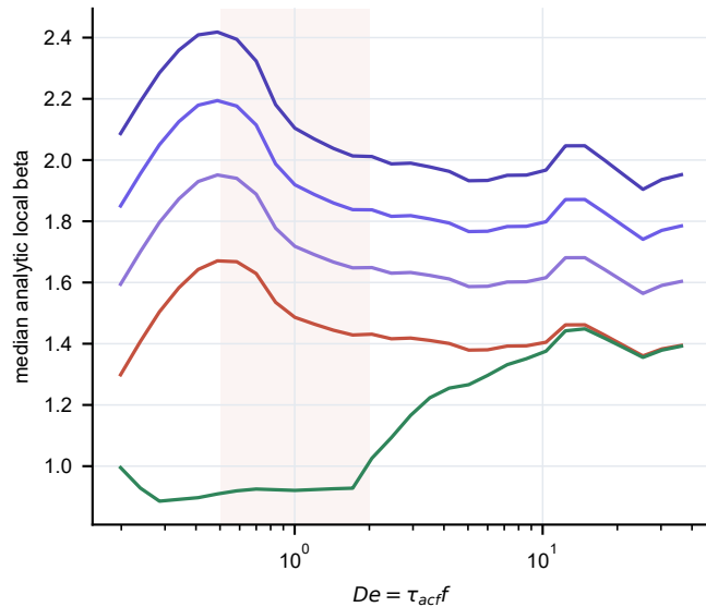
Gauge-matched analytic beta(De) curves
