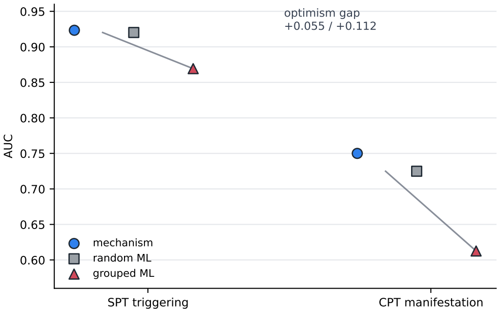
A Random validation inflates apparent ML skill
