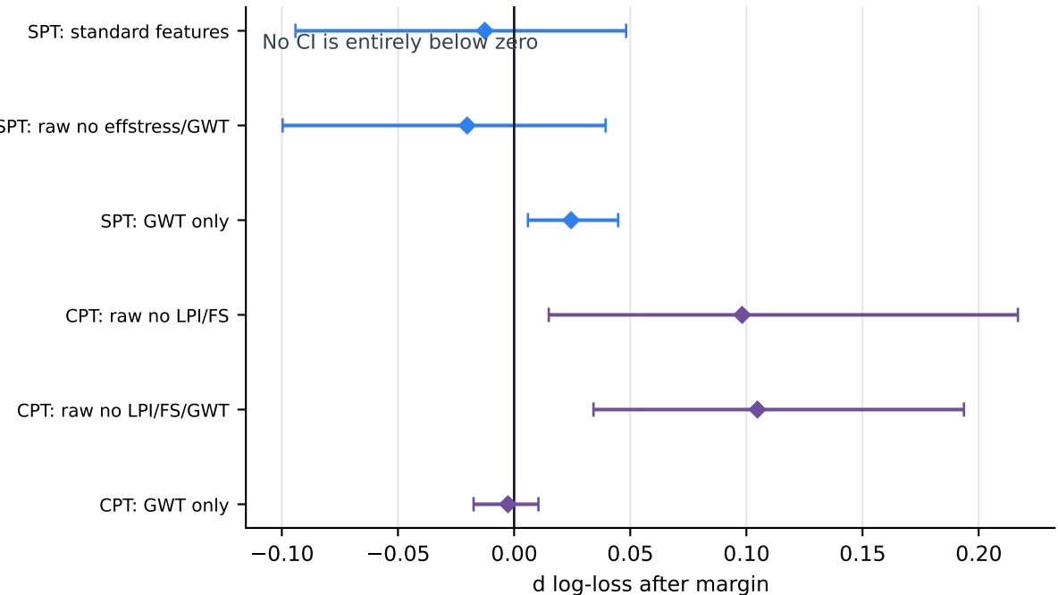
C Residual/raw variables after the margin
