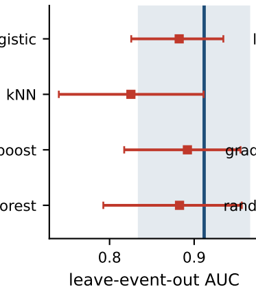
V_s (triggering); margin 0.912
