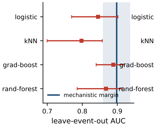
SPT (triggering); margin 0.898
