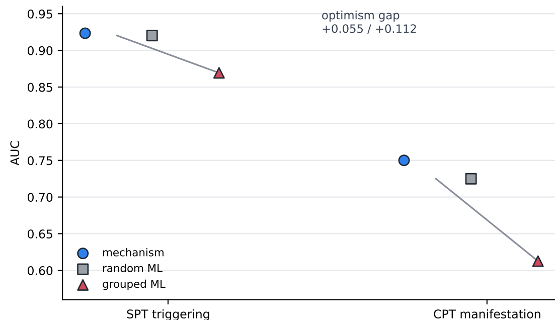
A Random validation inflates apparent ML skill
