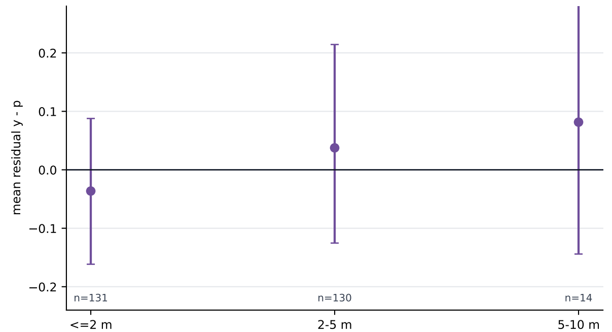
D CPT residuals by groundwater-depth bin
