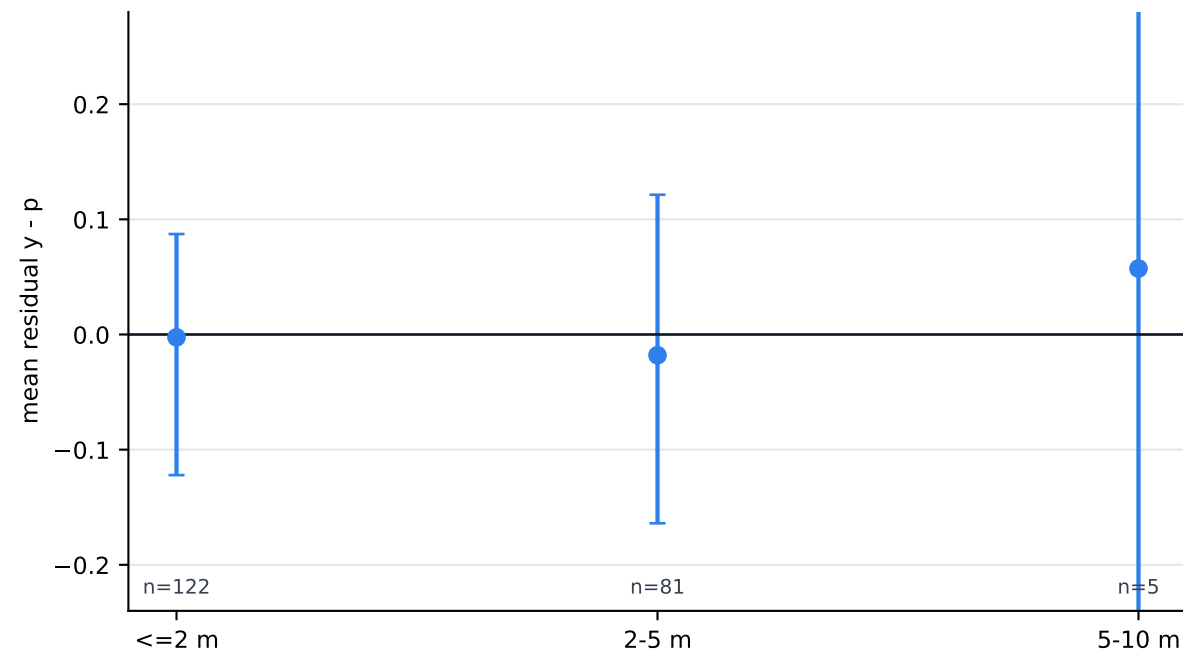
C SPT residuals by water-depth bin
