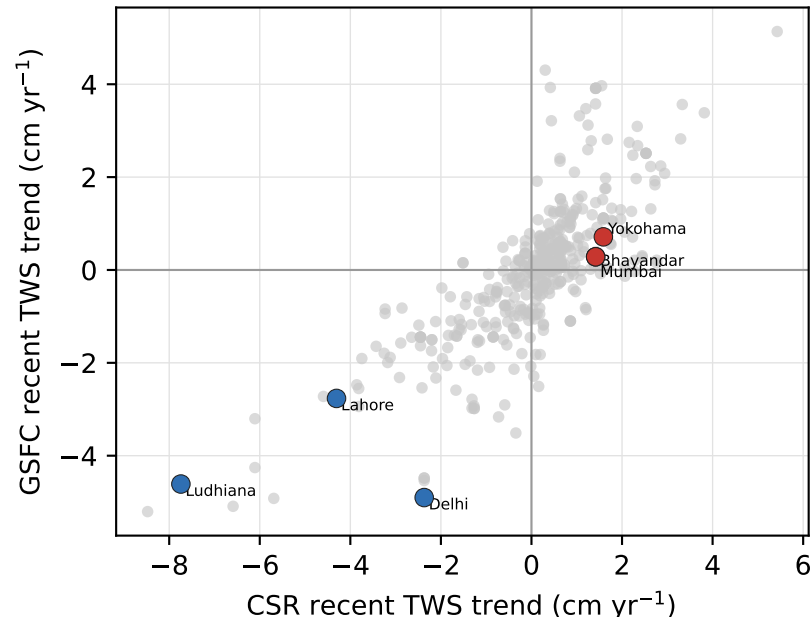
b Independent mascon sign check
