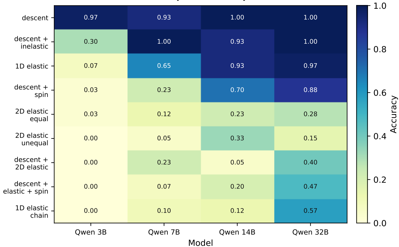
Family-level accuracy
