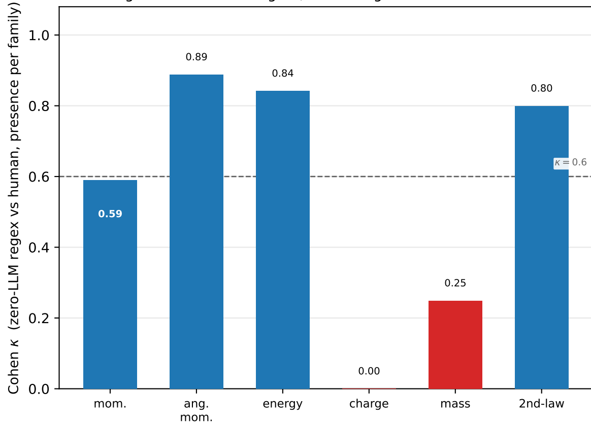
(b) Per-family agreement: zero-LLM regex vs human (n=1200) single-scalar families agree; rare charge/mass under-detected
