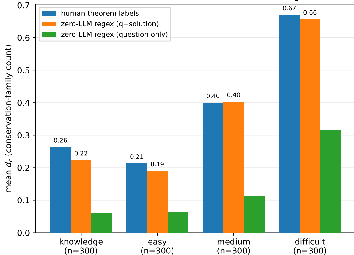
(a) Known-groups validity across PhysReason difficulty tiers human and zero-LLM labels track the same monotone gradient
