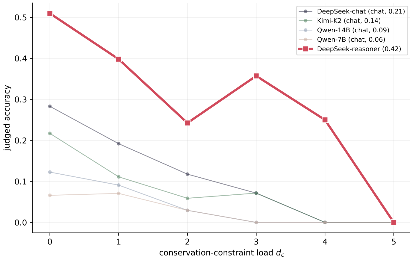
Strong-solver arm has real dynamic range and still declines with d_c DeepSeek-reasoner on full pilot258 (n=254); univariate OR per +1 d_c = 0.68
