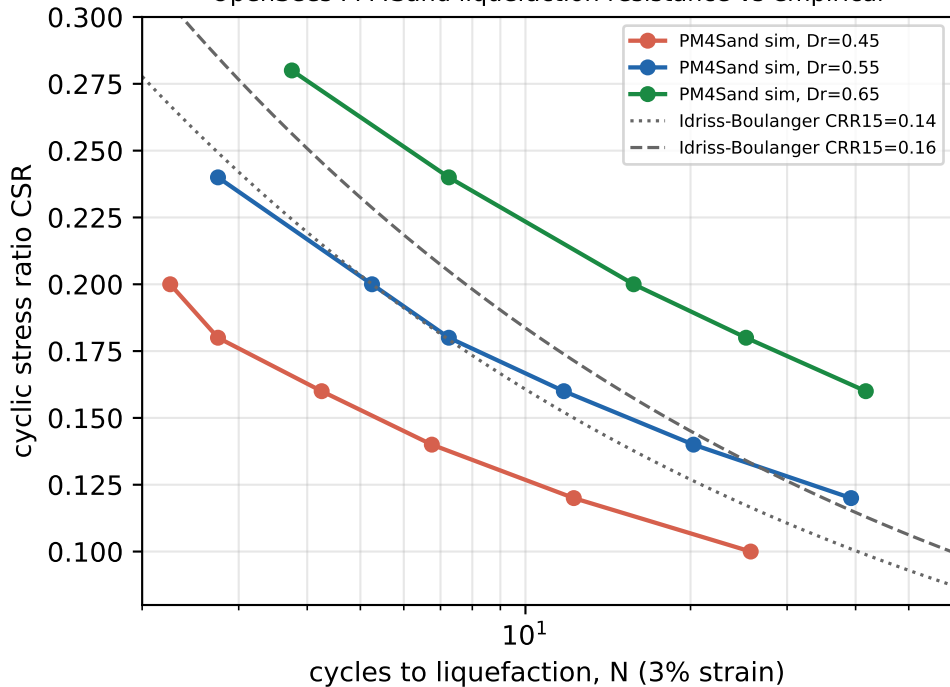
OpenSees PM4Sand liquefaction resistance vs empirical
