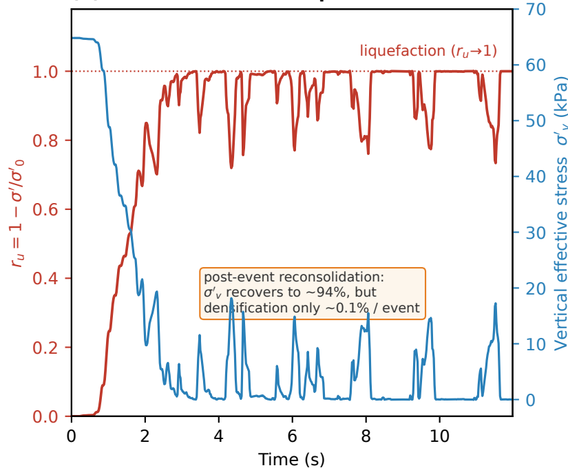
(B) Effective-stress collapse under one event
