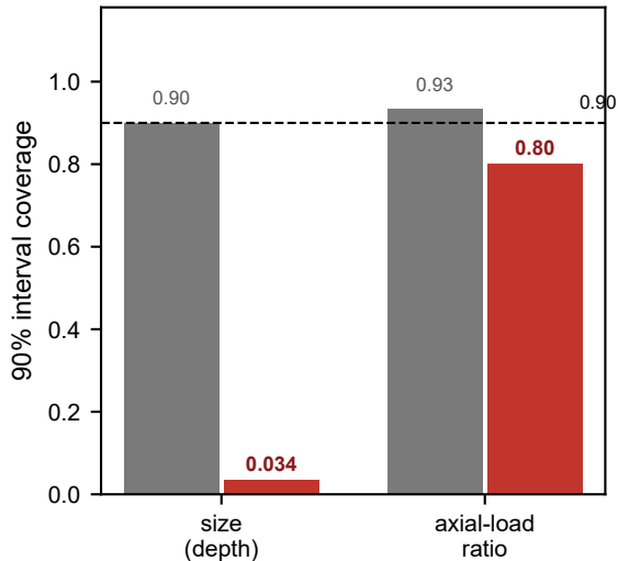
A RC columns (n=234): interval coverage falls out of envelope B
