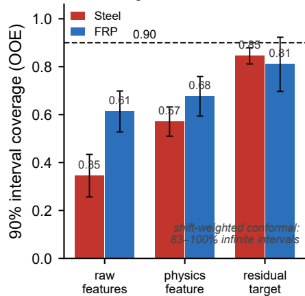
C Physics-anchored learning helps; the gate is still needed
