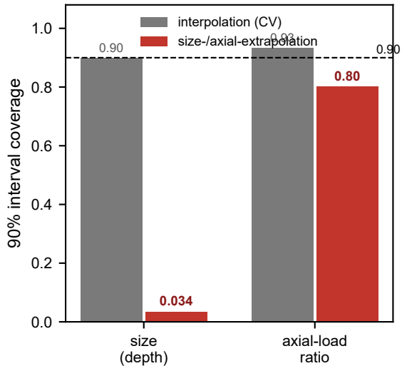
A RC columns (n=234): interval coverage falls out of envelope
