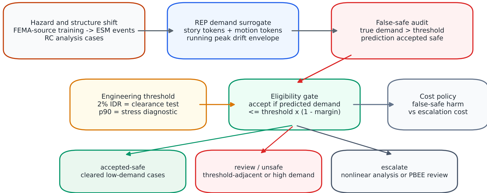
Figure 1. A selective decision architecture for seismic-demand screening under event-level source shift.
