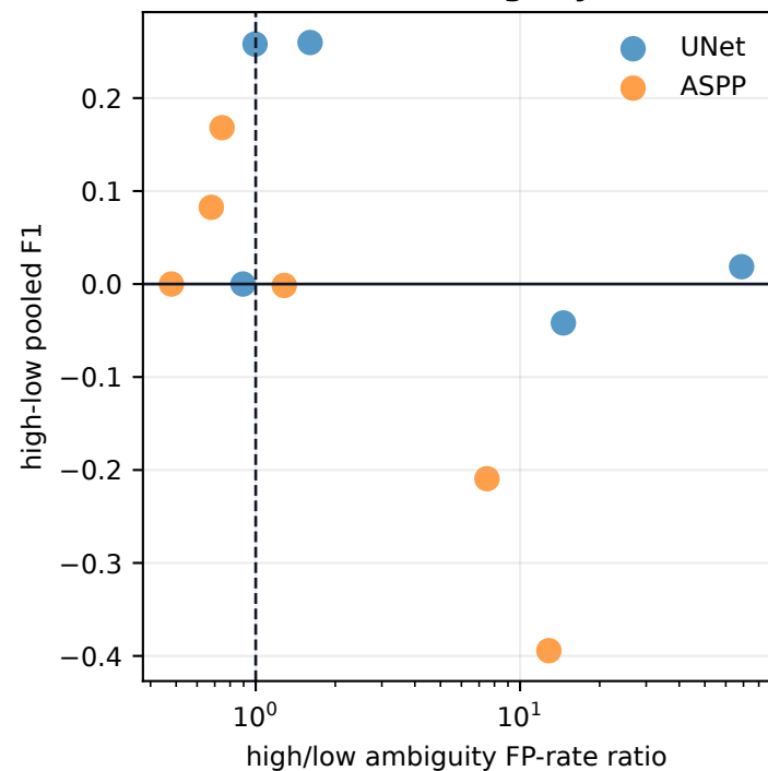
a Observation-ambiguity interaction
