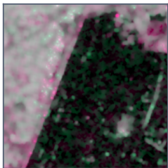
a VV/VH SAR composite
