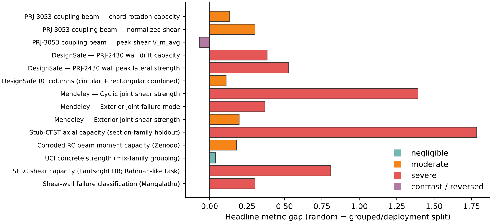
Random Forest headline gaps (nine reproduction modules)
