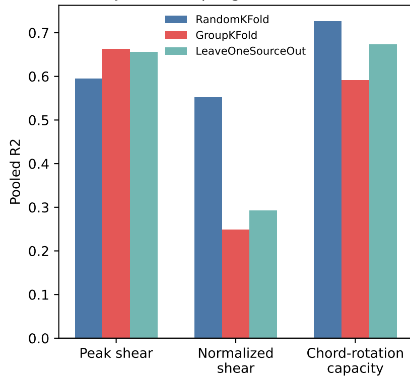
PRJ-3053 coupling beam validation
