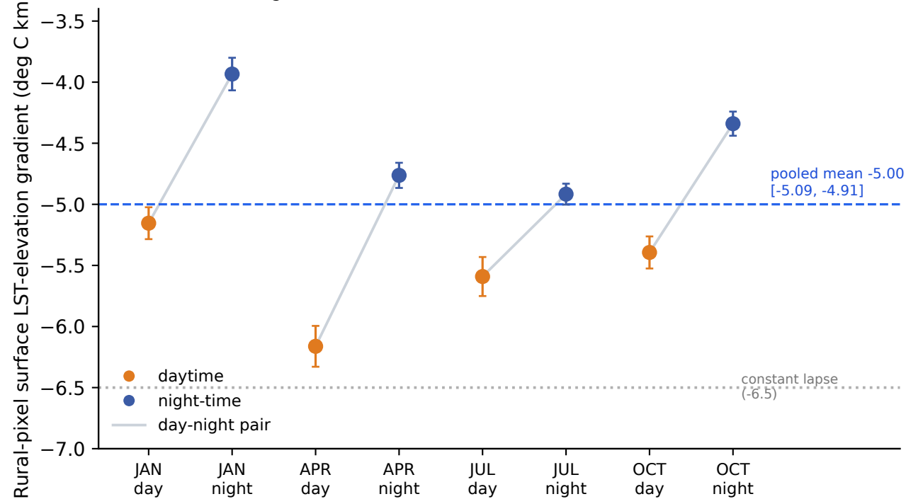
Rural LST-elevation gradients
