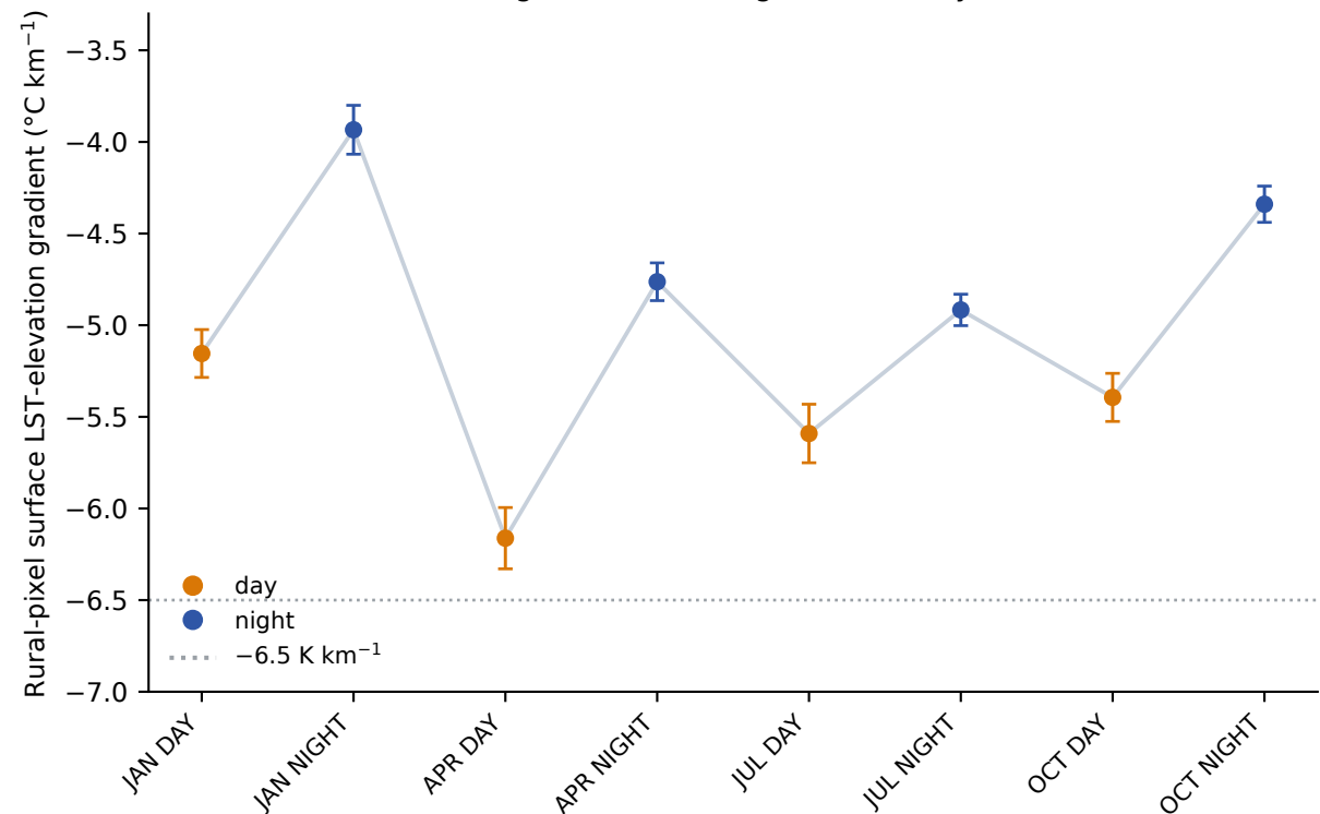
Pixel-scale LST-elevation gradients are negative in every window
