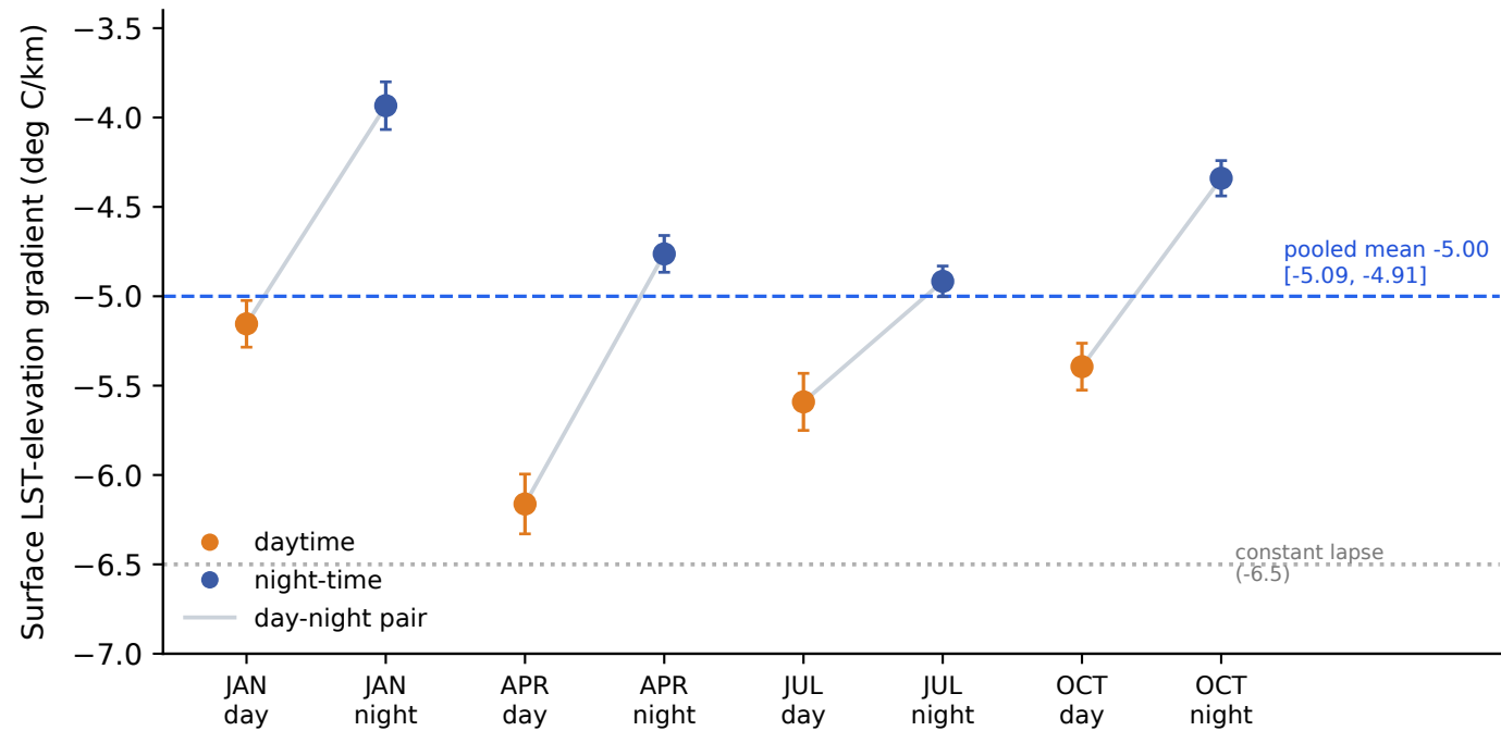
Rural LST-elevation gradients
