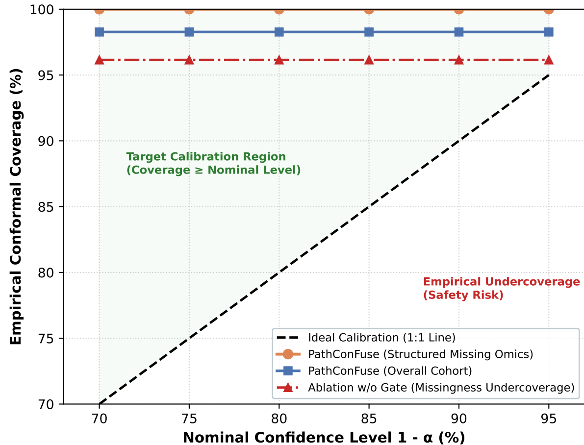
(b) Conformal Coverage Reliability & Calibration Curve
