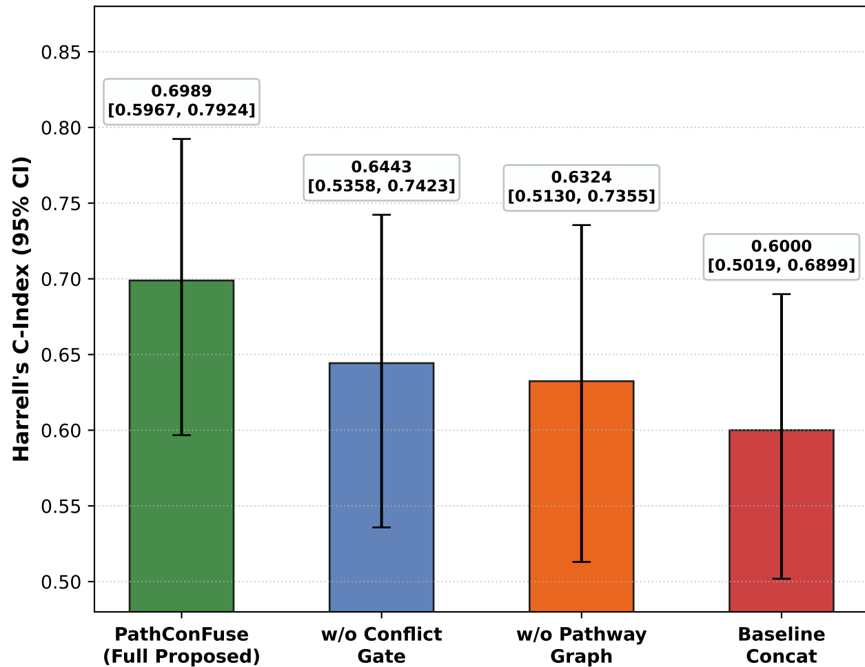
(a) Discriminative Performance Across Architectural Ablations
