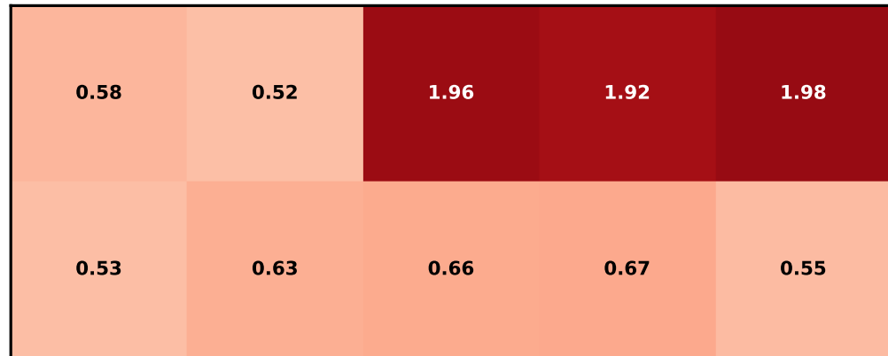
RET Mean Attention Heatmap
