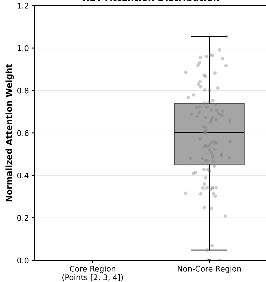
RET Attention Distribution
