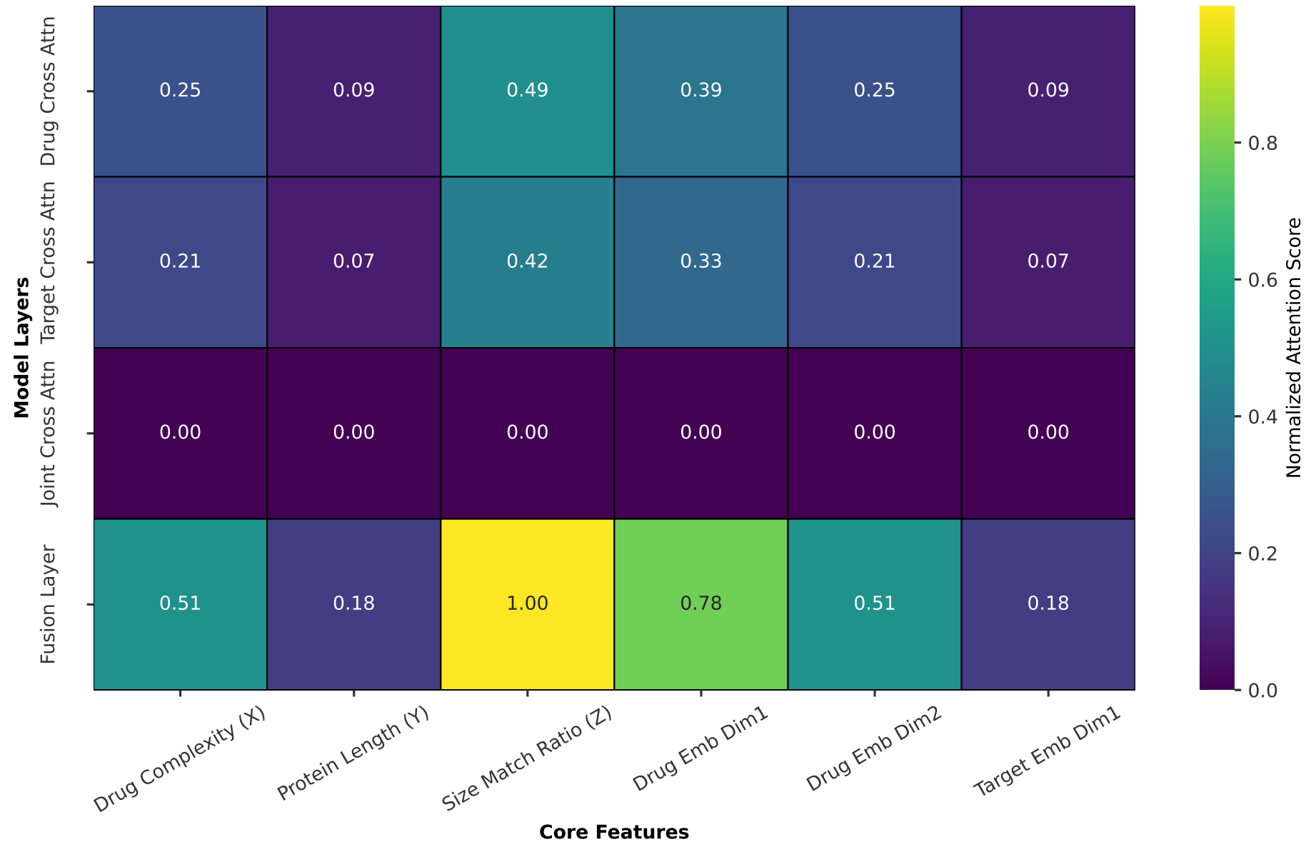
Layer-wise Attention on Core Features (DTA, Sample 100) (Core Point: 9th Point)
