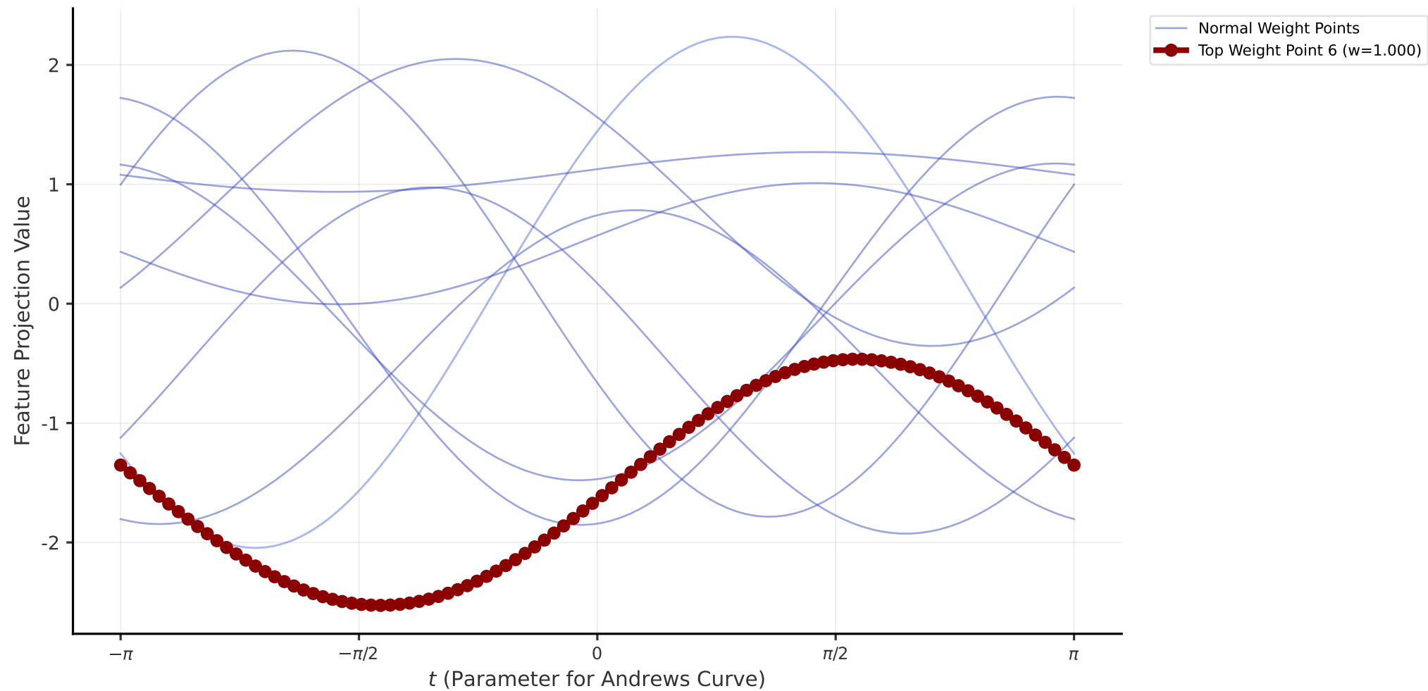
Andrews Curve of 10 Points (Sample 100, DTA Task)
