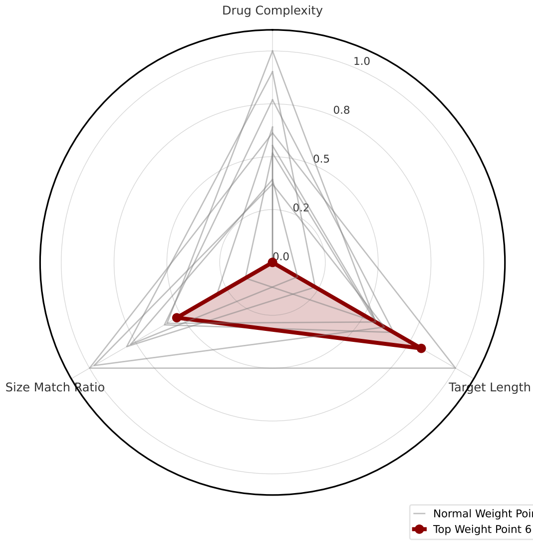
Feature Contribution (DTA Task, Sample 100)
