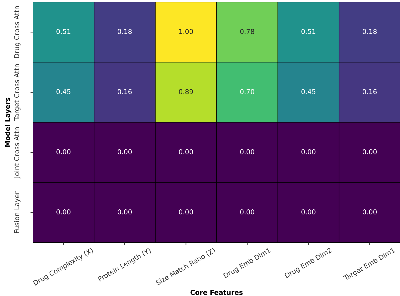
Layer-wise Attention on Core Features (DTA, Sample 100) (Core Point: 9th Point)
