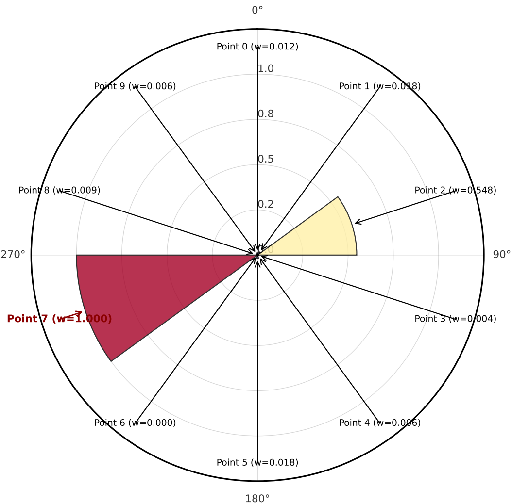
Attention Weights (DTI Task, Sample 100) Top Weight Point 7 (w=1.0000)
