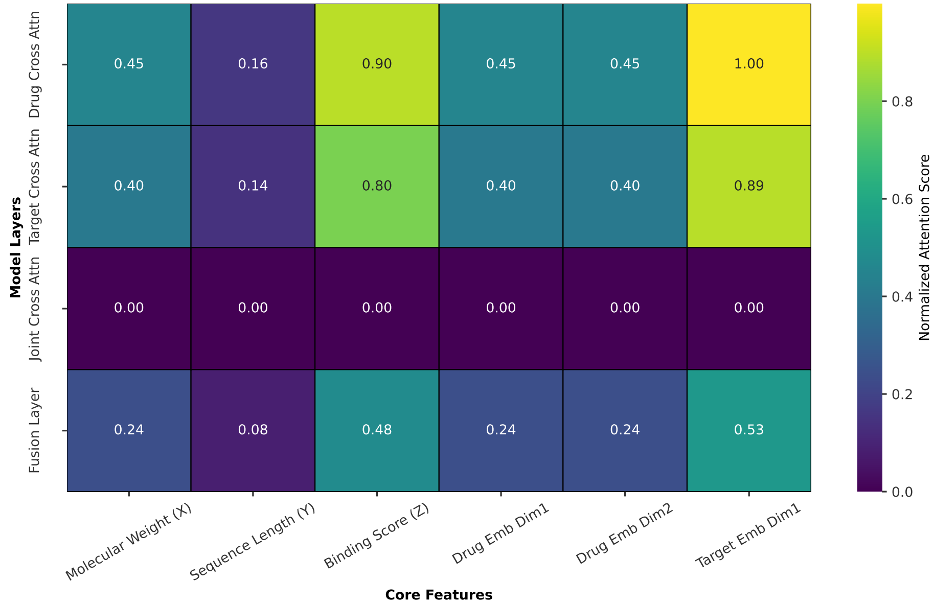
Layer-wise Attention on Core Features (DTI, Sample 100) (Core Point: 9th Point)
