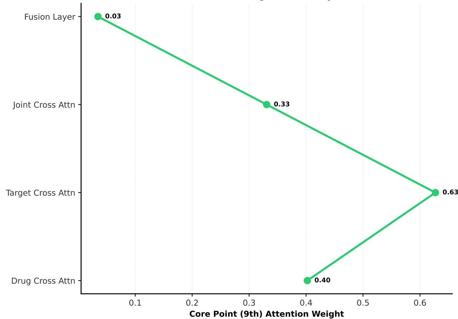
Core Point Weight Across Layers
