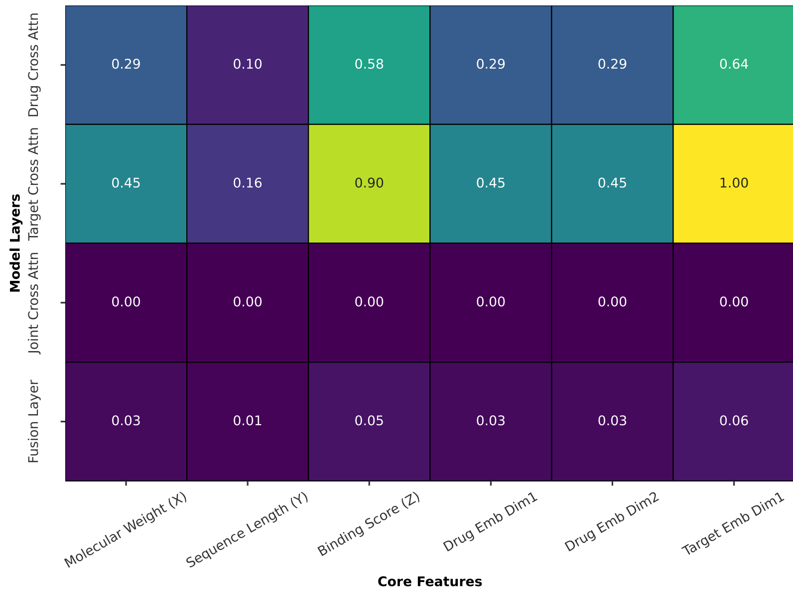
Layer-wise Attention on Core Features (DTI, Sample 100) (Core Point: 9th Point)
