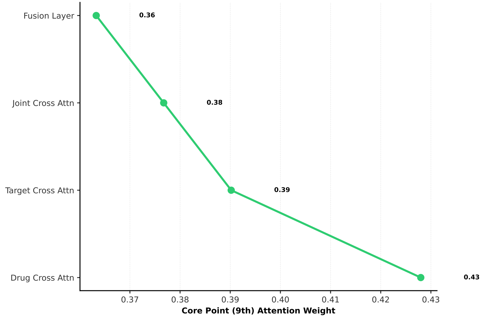
Core Point Weight Across Layers
