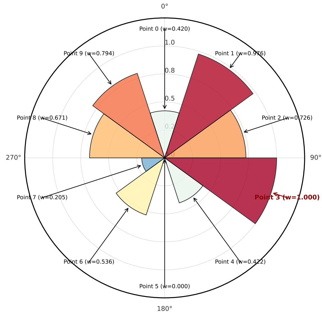
Attention Weights (DTI Task, Sample 100) Top Weight Point 3 ( w=1.0000 )
