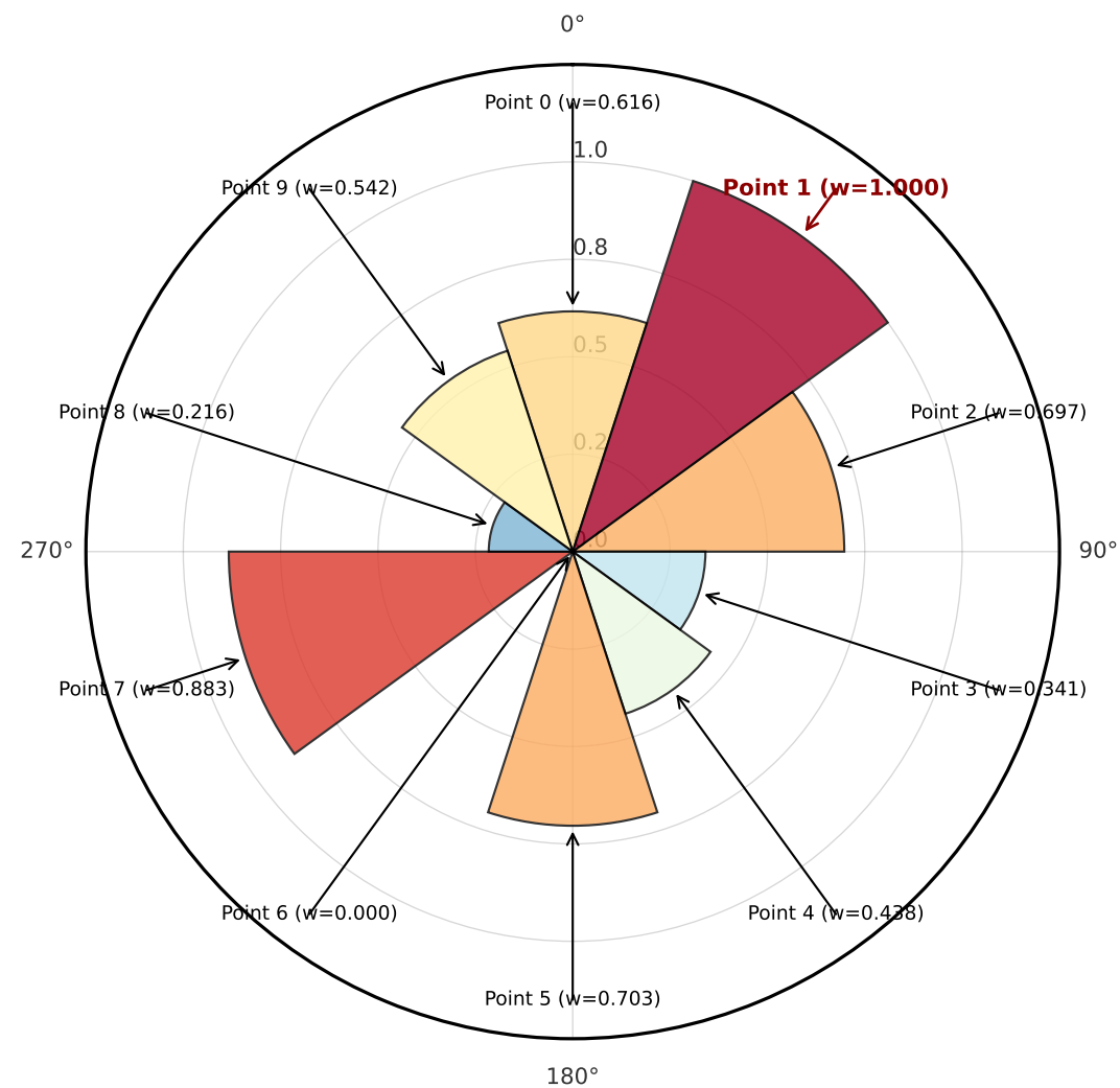
Attention Weights (DTI Task, Sample 100) Top Weight Point 1 (w=1.0000)
