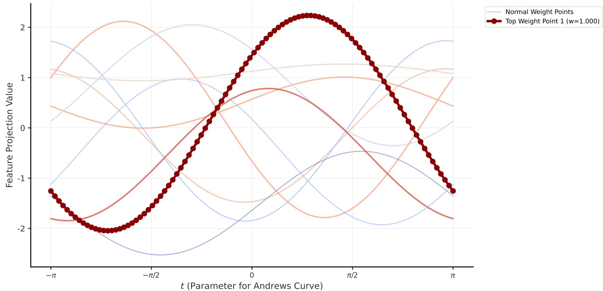
Andrews Curve of 10 Points (Sample 100, DTI Task)
