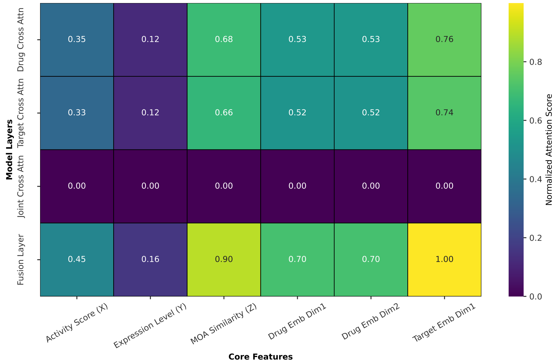
Layer-wise Attention on Core Features (MOA, Sample 100) (Core Point: 9th Point)
