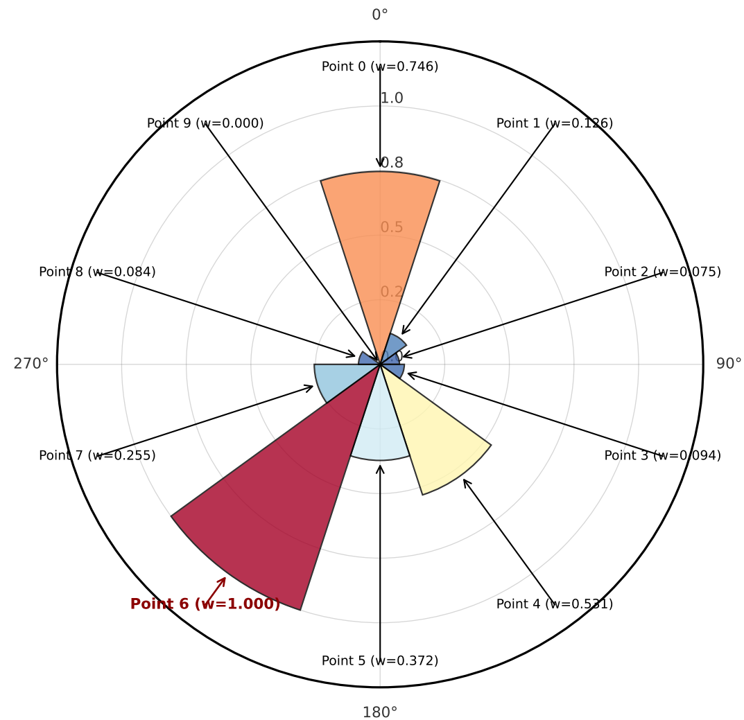
Attention Weights (MOA Task, Sample 100) Top Weight Point 6 ( w=1.0000 )
