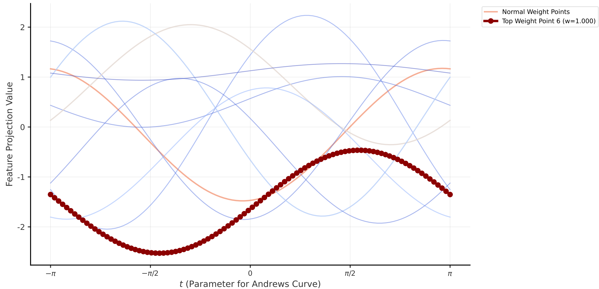
Andrews Curve of 10 Points (Sample 100, MOA Task)
